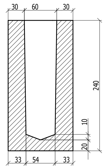
B-B (1:4)
